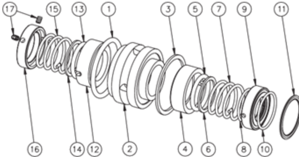
Breakdown For LC/LD Series Pumps (Items 12-17 for LD Series Pumps only)
